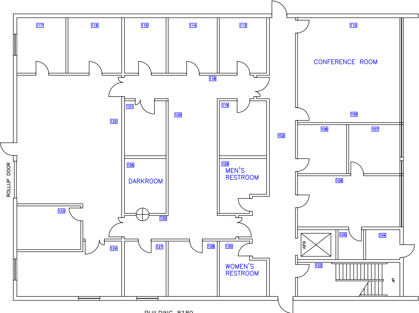
BUILDING 8189 FIRST FLOOR - MATERIALS PROCESSING LABORATORY
